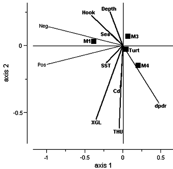
Fig. 7 RDA biplot for acoustic data from vessel V7 (Brazil). Response variables (represented by thin lines): likely delphinid clicks (Pos) and unlikely delphinid clicks (Neg). Explanatory variables (represented by thick lines if continuous and by squares if nominal): see Table 4. The plot shown was based on re-running the RDA having removed the least important (non-significant) explanatory variables, to achieve greater visual clarity
